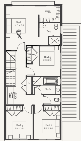
FIRST FLOOR 4 BEDROOM PLAN
